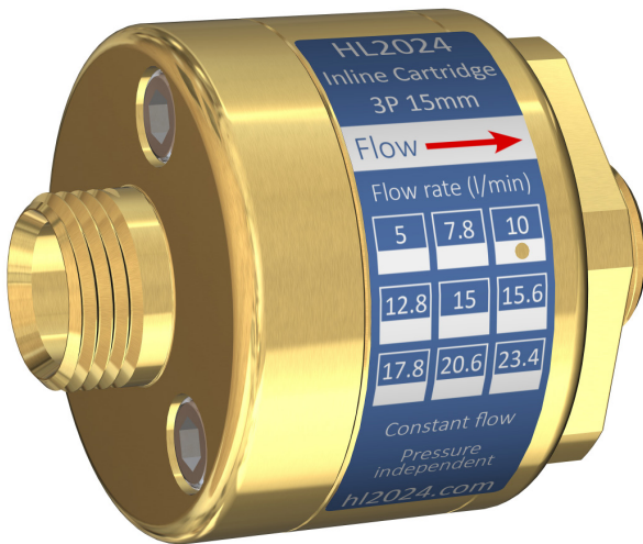
Top left: HL2024 Inline Cartridge 3P 15mm
